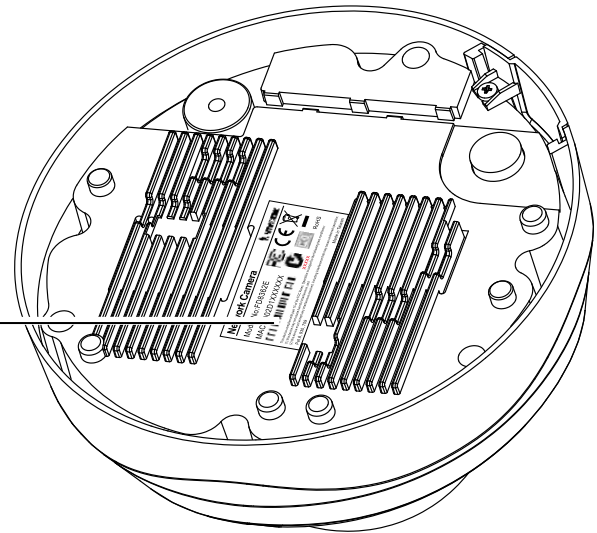
Mounting Plate
