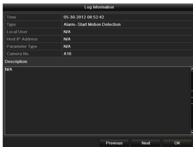
Figure 12. 9 Log Details
