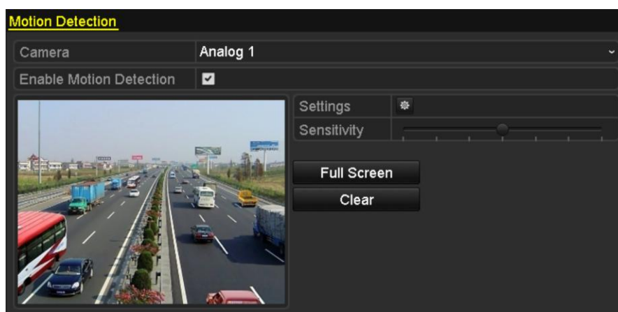
Figure 5.15 Motion Detection
