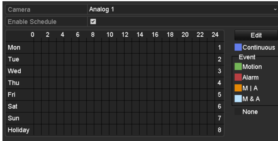
Figure 5. 17 Record Schedule
