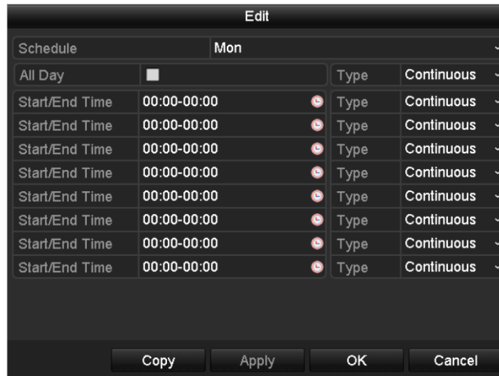
Figure 5. 9 Edit Schedule
