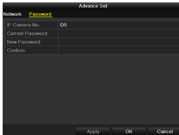
Figure 2. 19 Advance Set-Password
