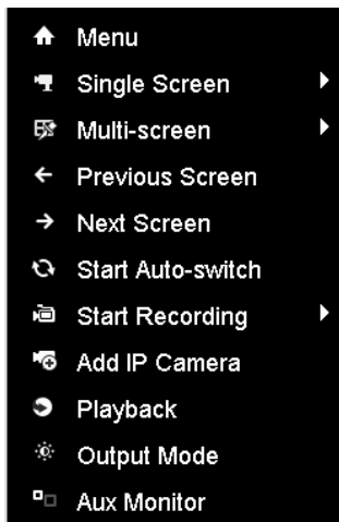
Figure 3. 1 Right-click Menu
