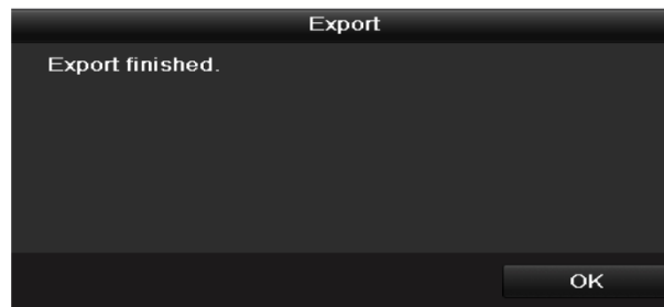
Figure 7. 15 Export Finished
