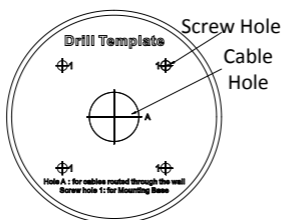
Figure 2-5 The Drill Template
