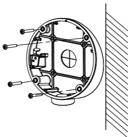
Figure 2-7 Fix the Inclined Ceiling Mount's Body
