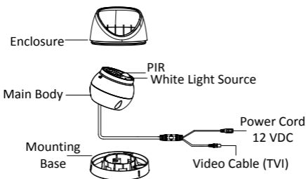
Figure 1-1 Overview of Type I Camera
